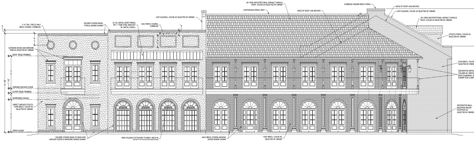
RYAN STREET VIEW- WEST ELEVATION
