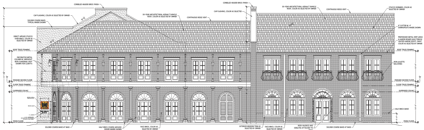
KIRBY STREET VIEW-- SOUTH ELEVATION
